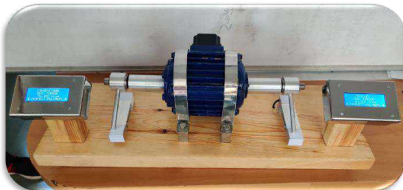
Torque Testing System
